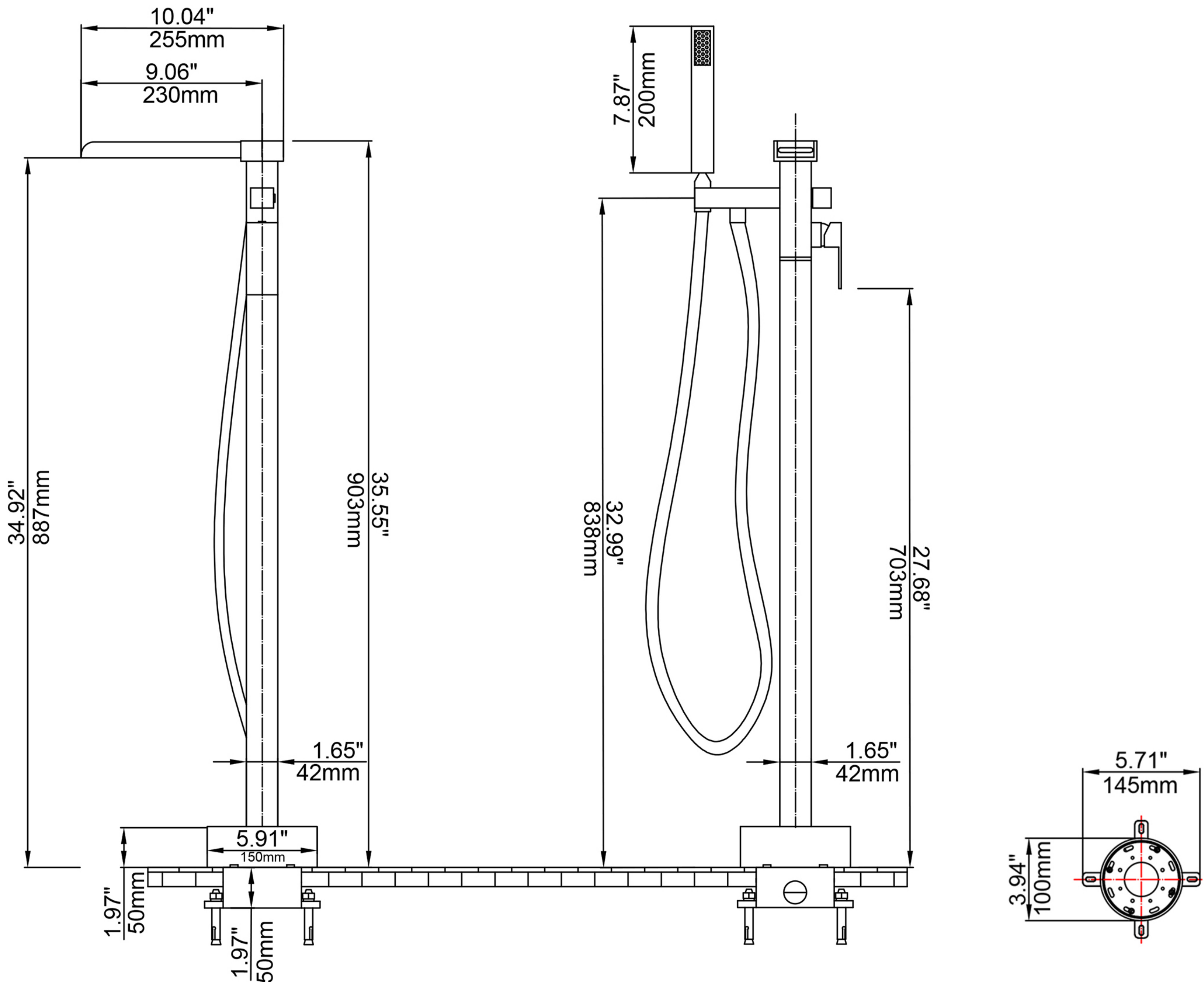
CRITICAL DIMENSIONS
