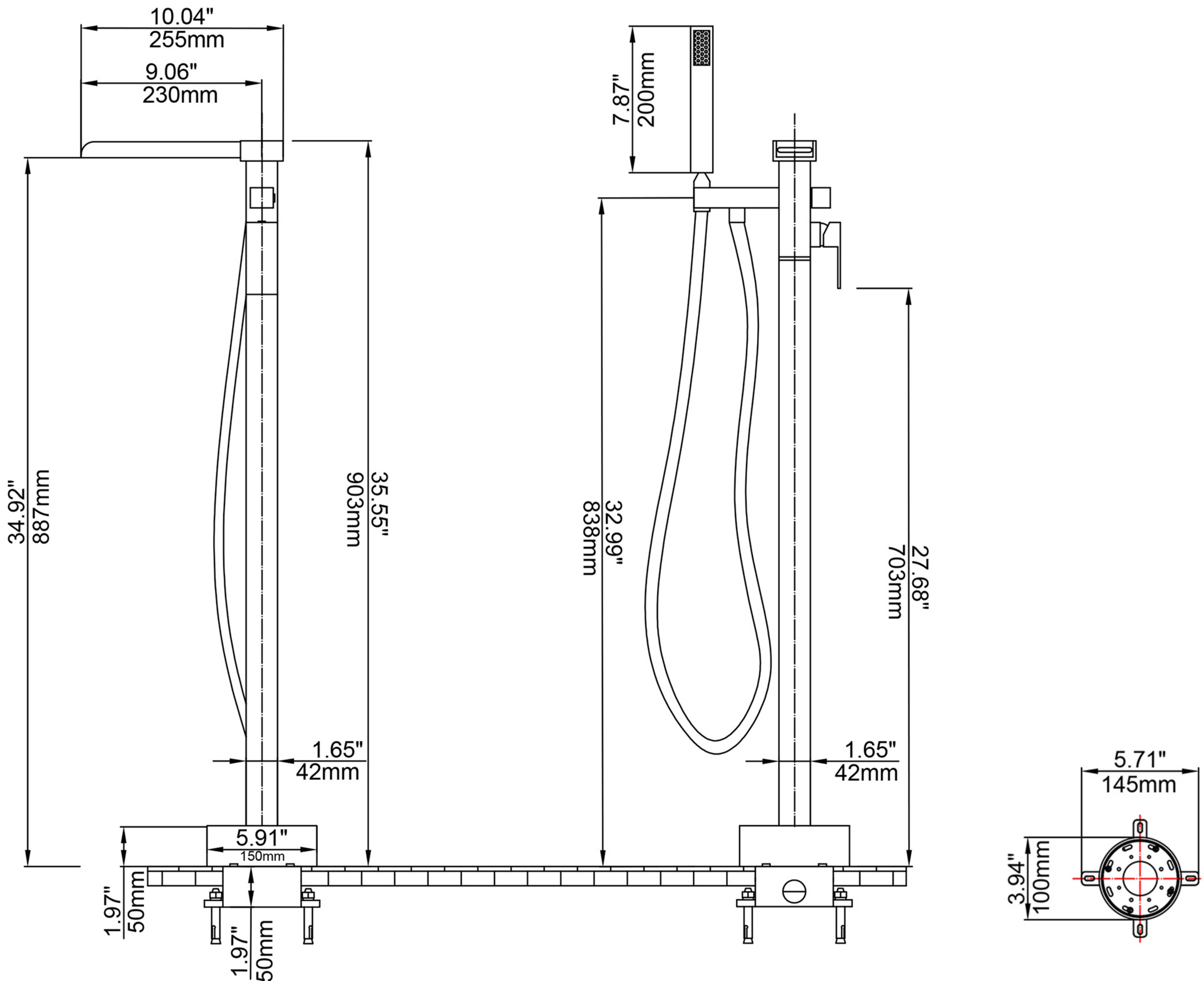
CRITICAL DIMENSIONS
