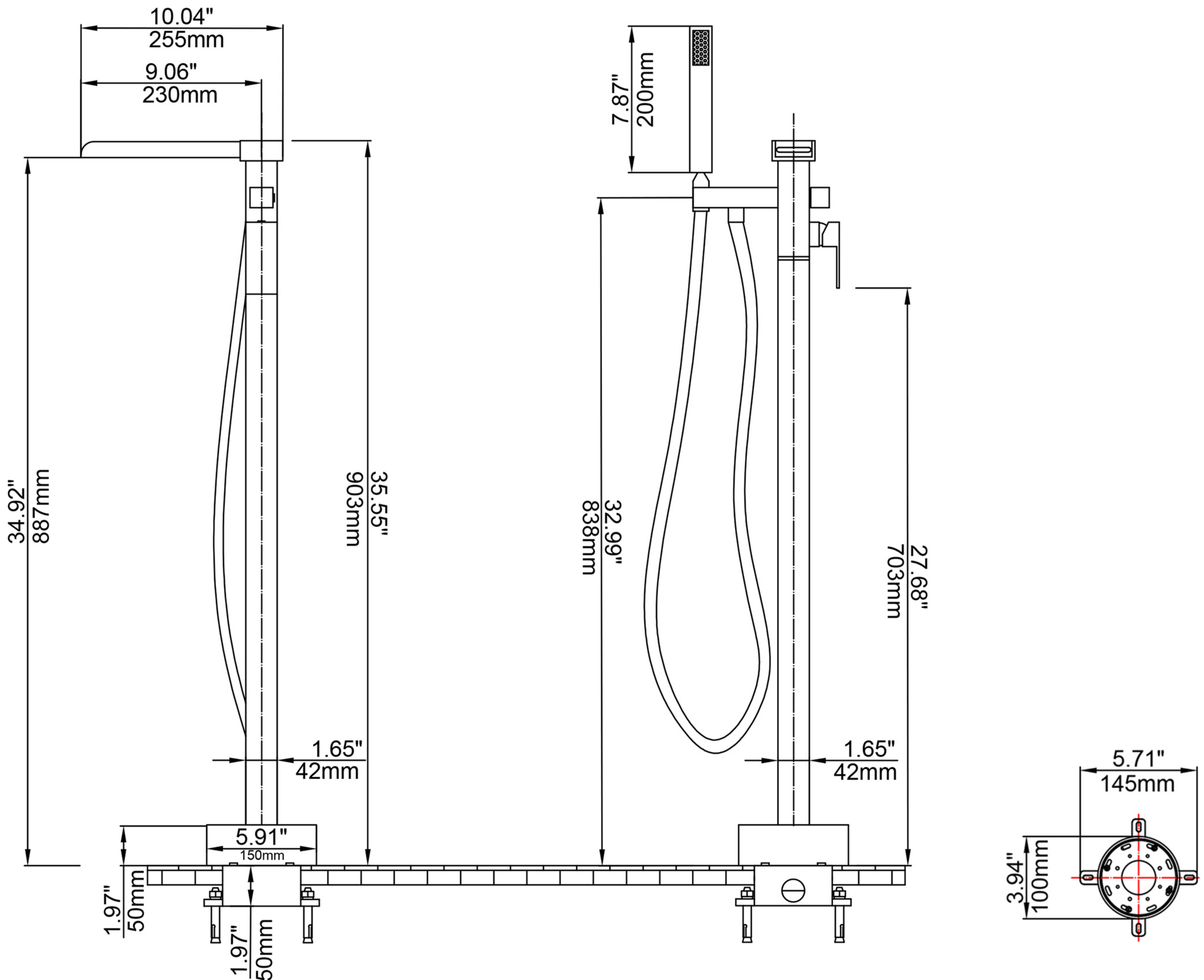
CRITICAL DIMENSIONS
