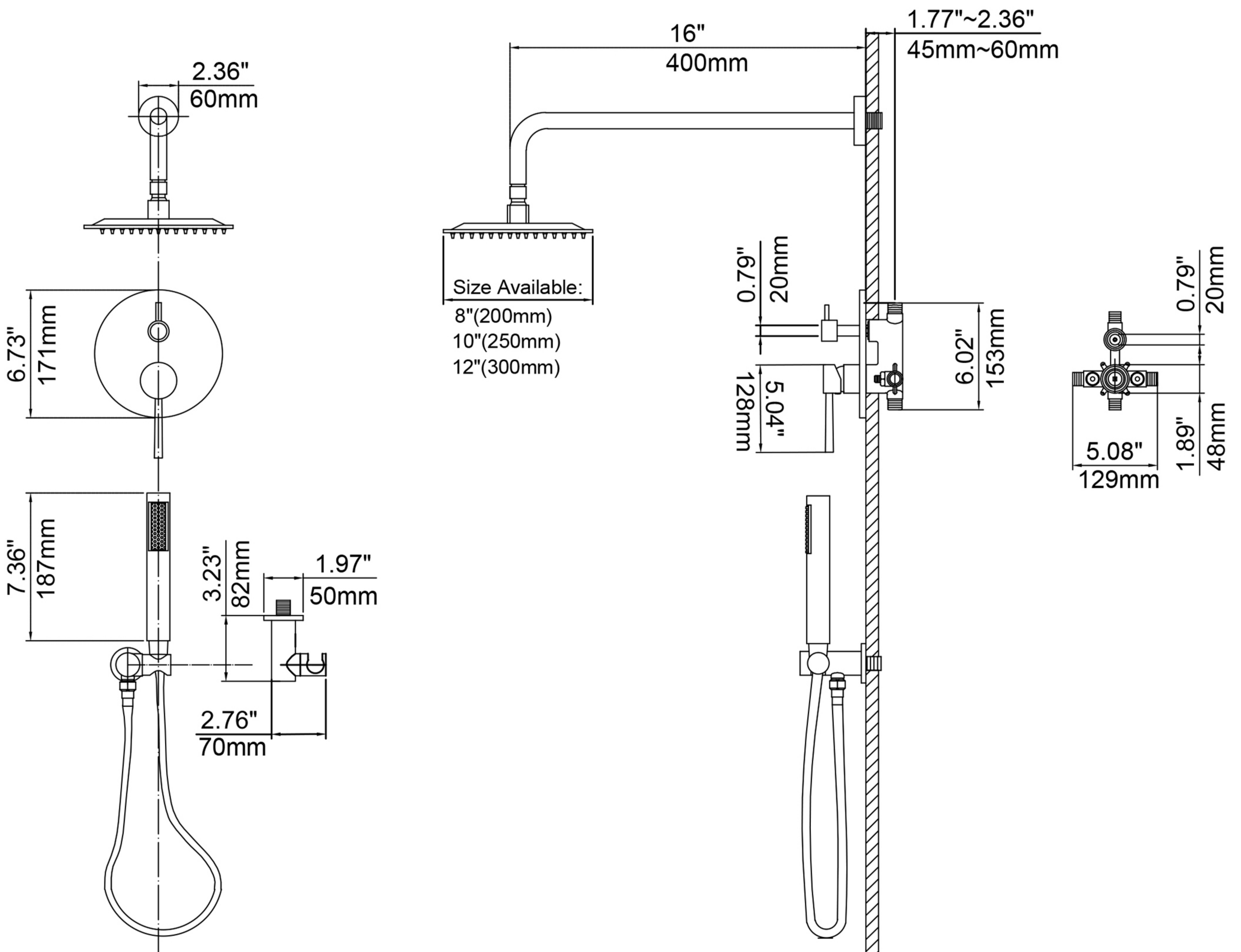
CRITICAL DIMENSIONS
