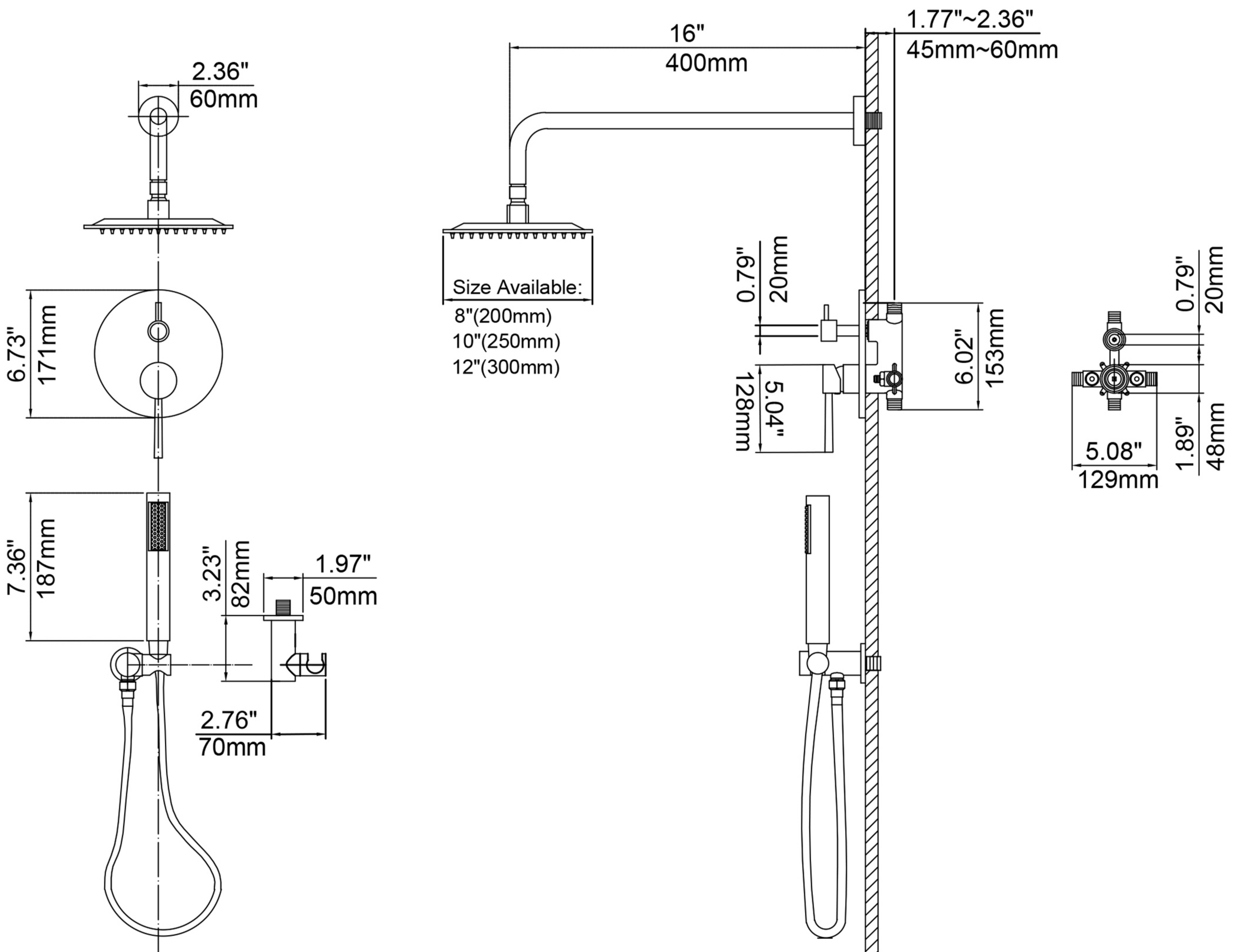
CRITICAL DIMENSIONS
